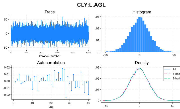
Figure 3 MCMC convergence
